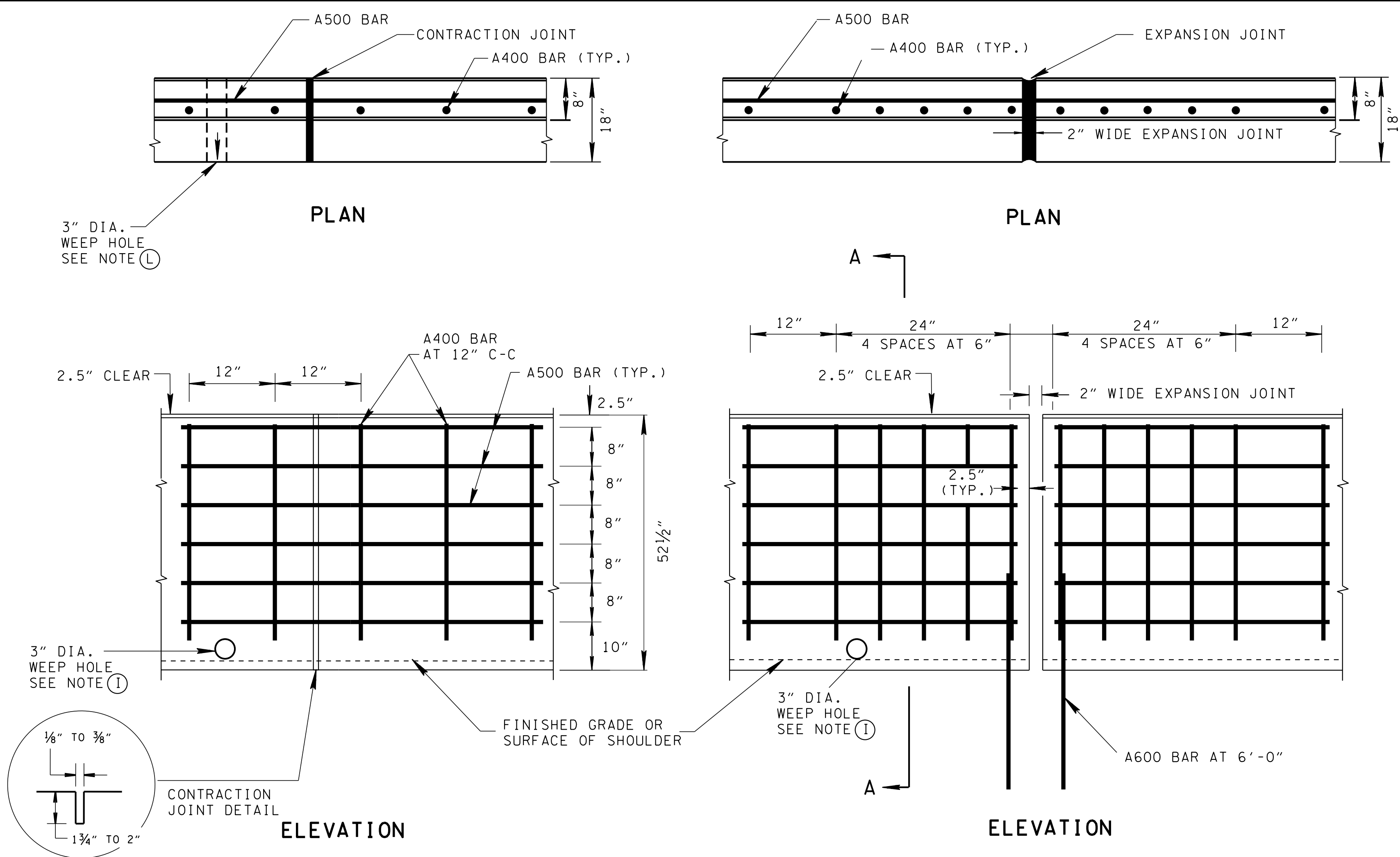
DETAILS OF REINFORCING AT CONTRACTION JOINT FOR CONCRETE BARRIER
