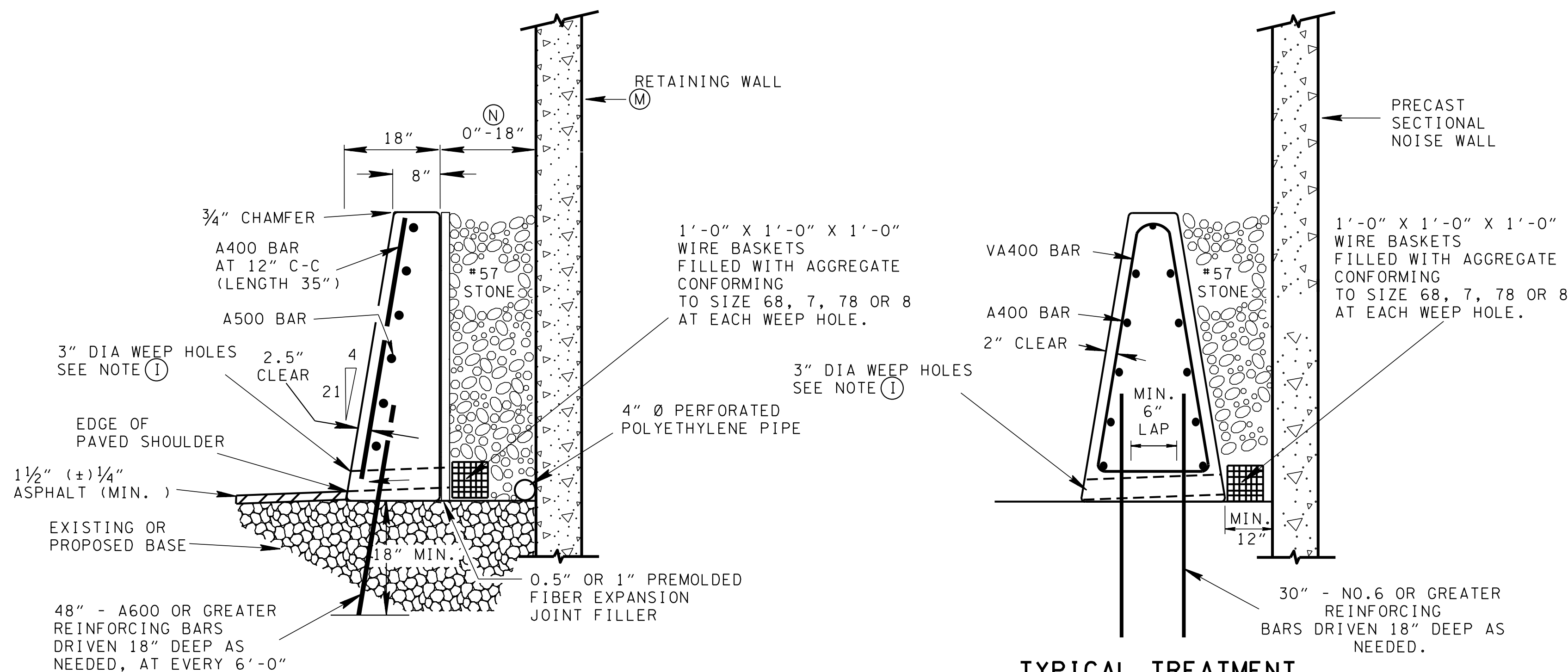
REINFORCING STEEL AT SECTION A-A (AT RETAINING WALL)
